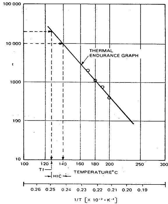
Figure A.1—Thermal endurance graph, TI, and HIC
